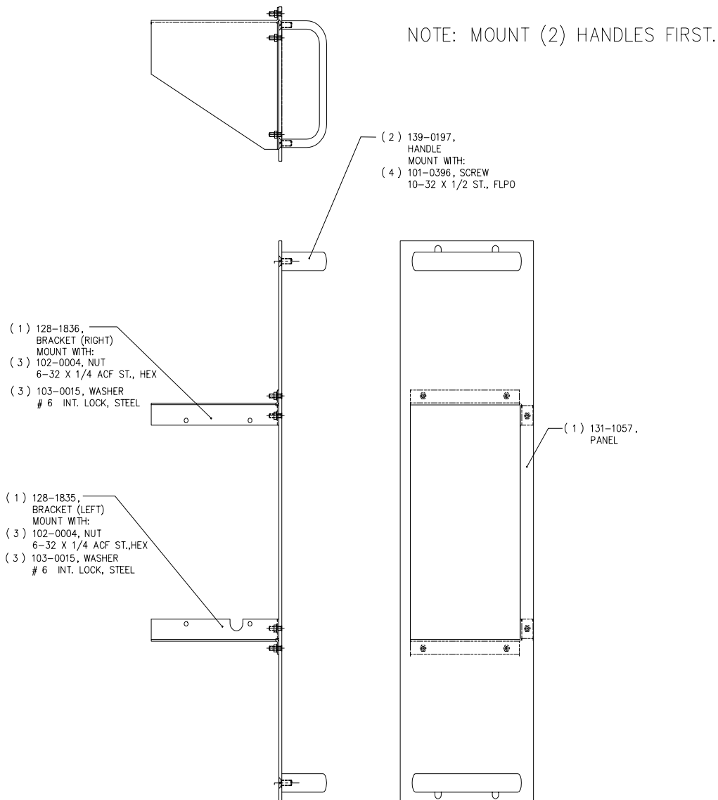
FIGURE 1. RA 71 RACK ADAPTER ASSEMBLY
